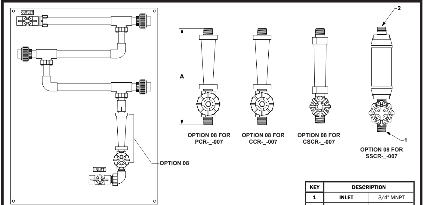
EXAMPLE OF OPTION 08 INSTALLED ON PCR-3-007/08
