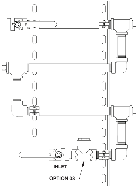
EXAMPLE OF OPTION 03 ON SSCR-3-007/03
